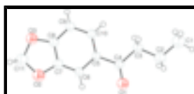
Fig. 1. The molecular structure of the title molecule, with the atom-numbering scheme.
